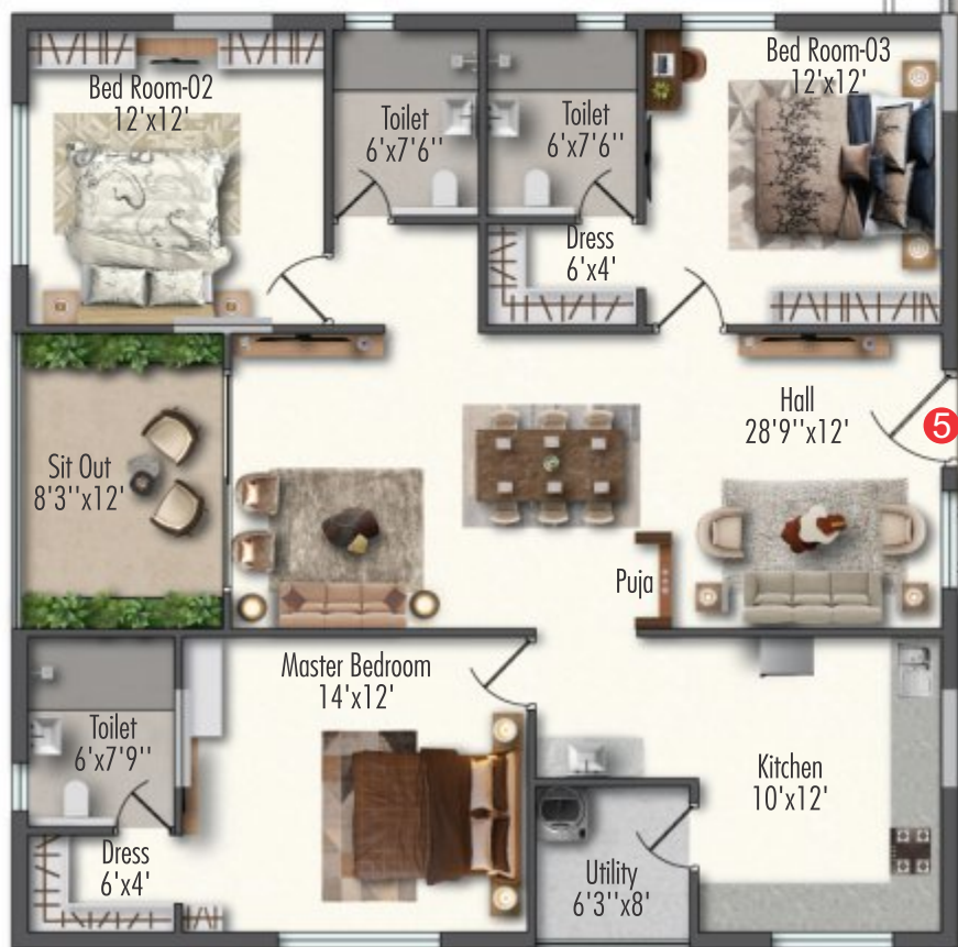
3 BHK-E-1850 Sft.
