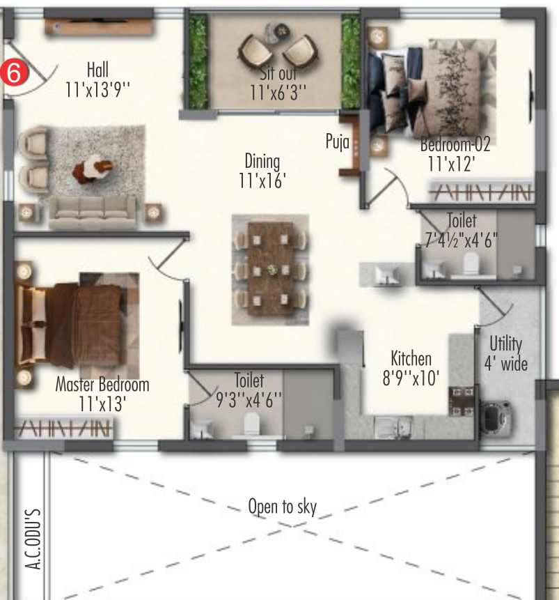
2 BHK-W-1250 Sft.
